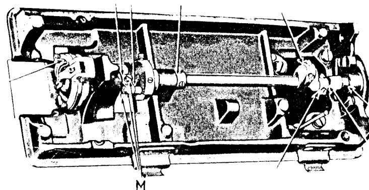
Fig. 6. Oiling Points and Adjustment Underneath the Machine
