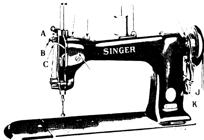
Fig. 3. Oiling Points and Adjustments at Front of Machine
