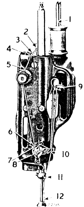
Fig. 8. Upper Threading
