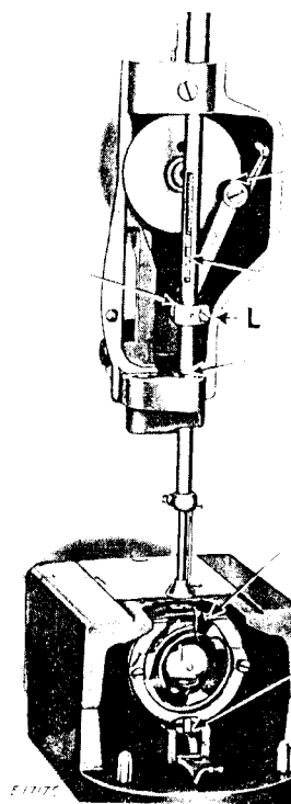
Fig. 5. Oiling Points at End of Machine
