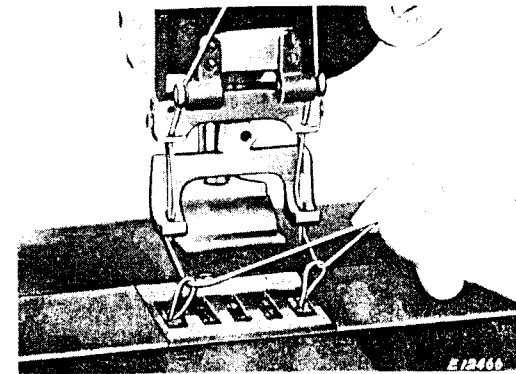
Fig. 13. Pulling Up the Bobbin Thread
