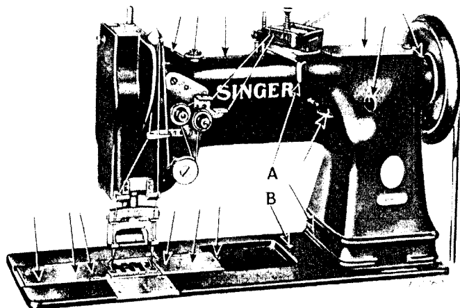
Fig. 2. Front View of Machine Showing Oiling Points
