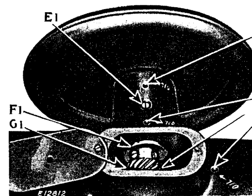
Fig. 26. Adjustments and Oiling Points at Top of Long-Arm Machines
