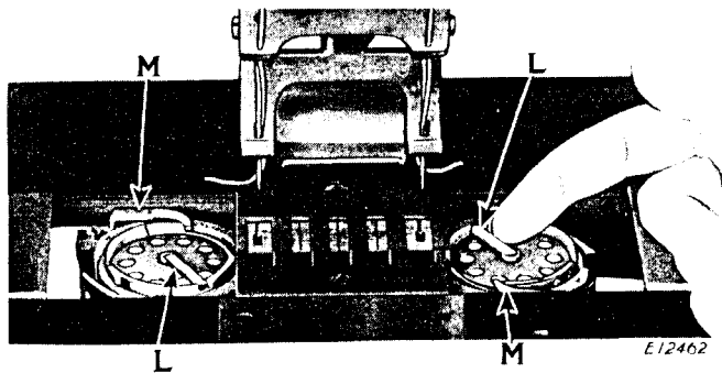
Fig. 7. Removing the Bobbin
