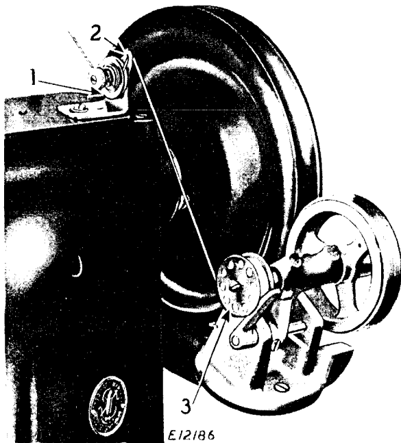
Fig. 9. Winding the Bobbin
