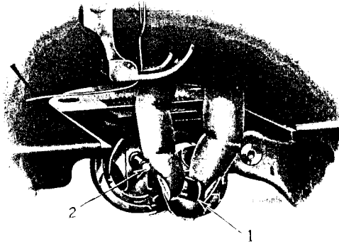
FIG. 3. REMOVING THE BOBBIN
